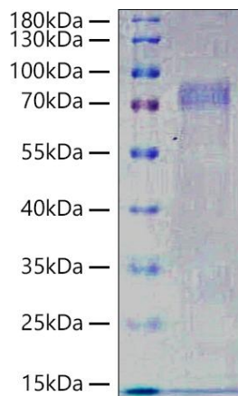
Figure 1. SDS-PAGE
